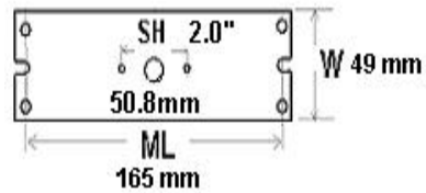
Series C1S Bottom Mounting
