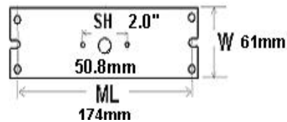
Series C2S Bottom Mounting
