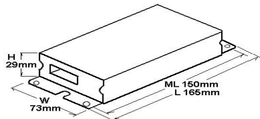
Series C4U Without Leads
