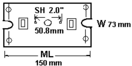
Series C4U Bottom Mounting
