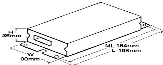
Series C7U Without Leads
