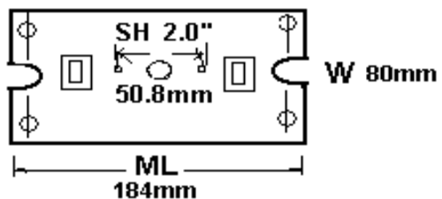
Series C7U Bottom Mounting
