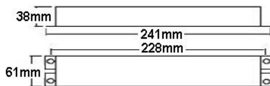
Series FS, KFS With Leads
