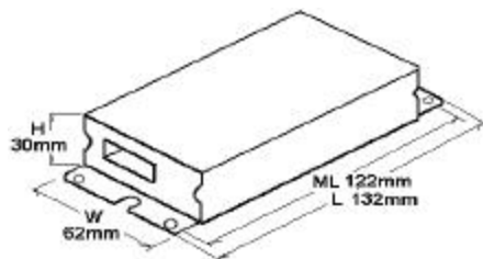
Series C1U Without Leads
